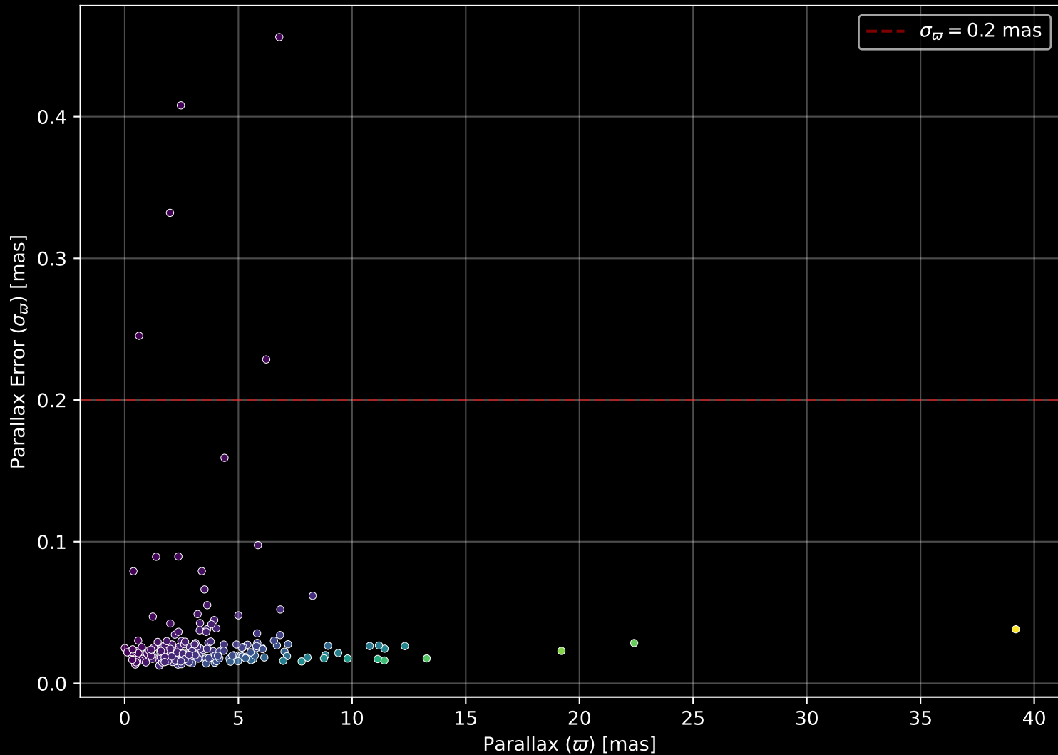
APOGEE DR17 Field: [K2_C12_089-63_btx] Parallax Quality (n= 201)
