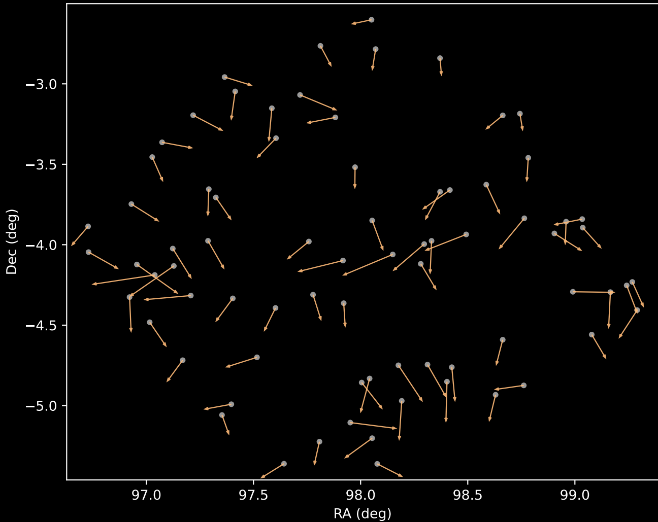
APOGEE DR17 Cluster 3 Proper Motion Vectors (n=75)
