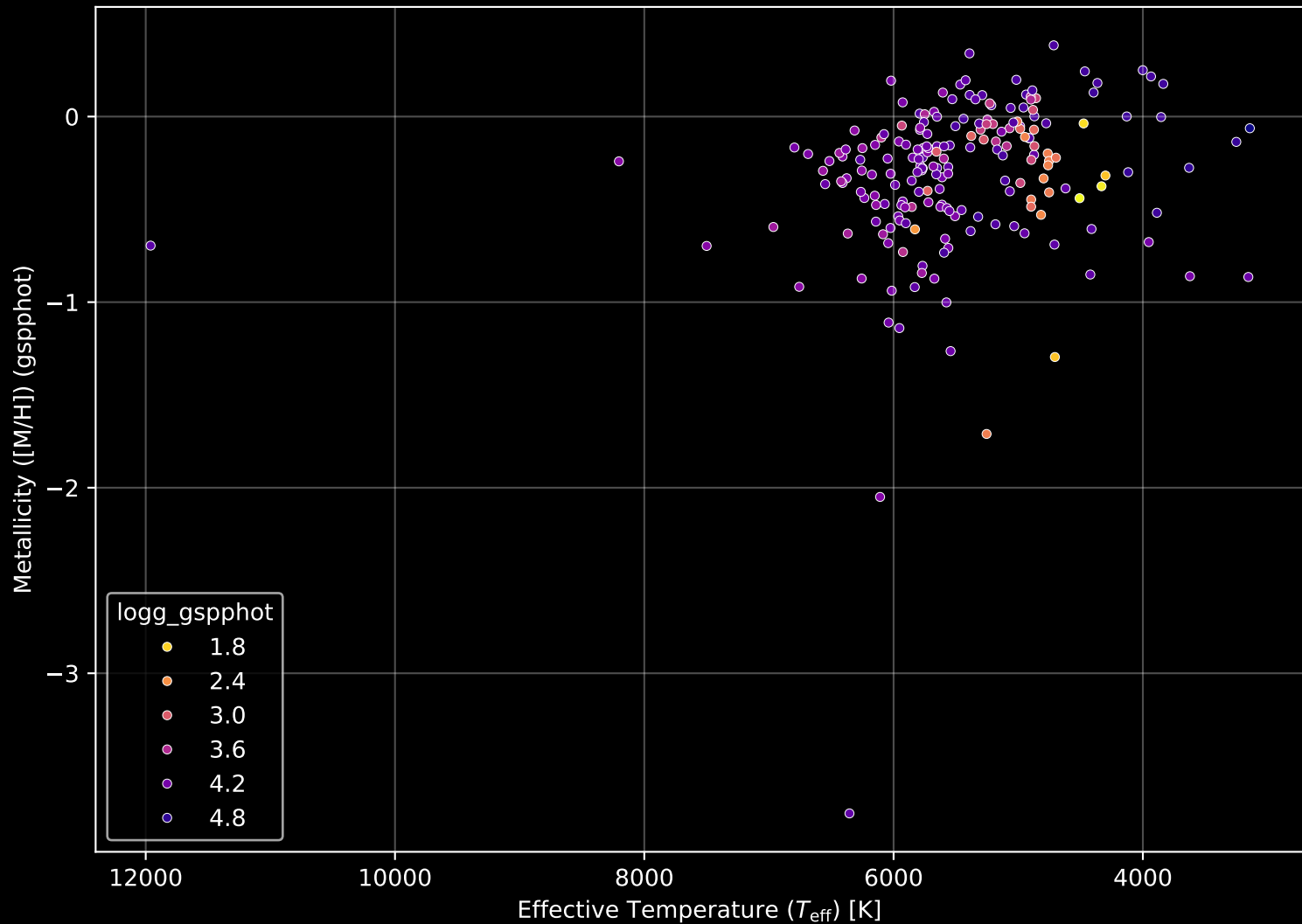
APOGEE DR17 Field: [K2_C12_089-63_btx] Stellar Population Parameters (n= 201)
