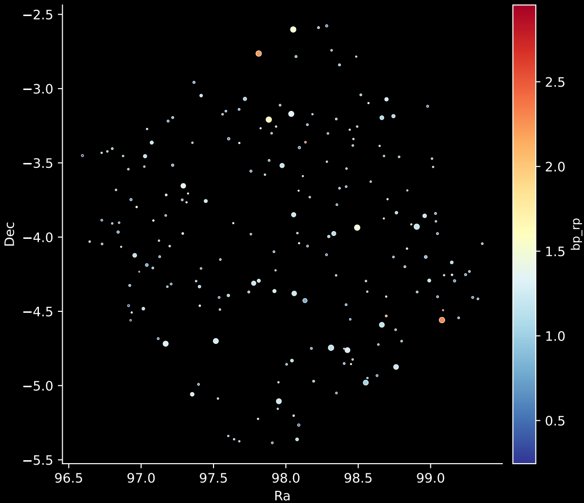
APOGEE DR17 Field: [K2_C12_089-63_btx] Stars: 201
