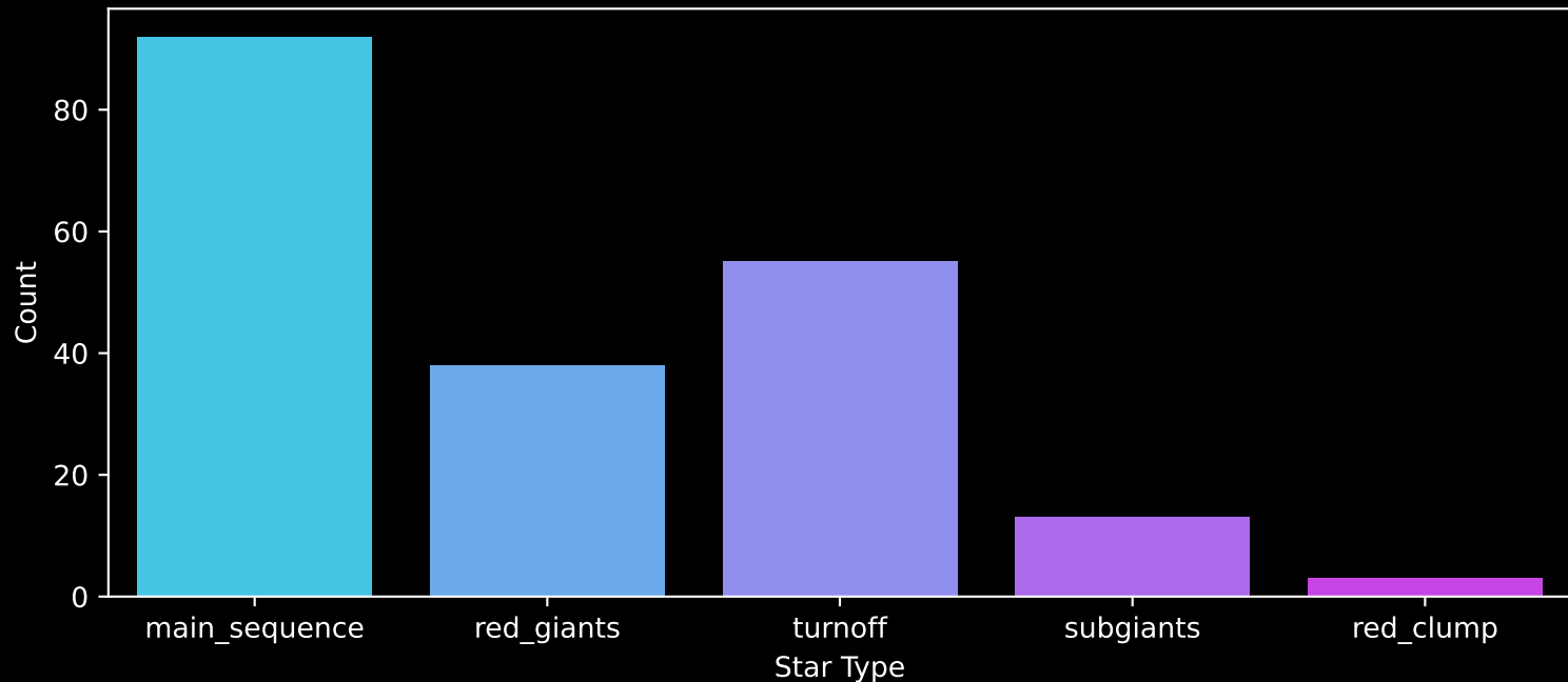
APOGEE DR17 Field: [K2_C12_089-63_btx] Count plot of Star Type
