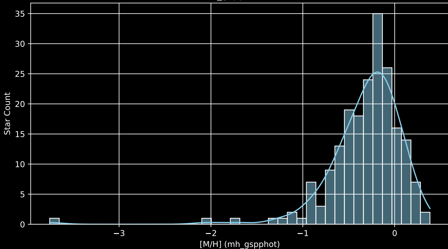
APOGEE DR17 Field: [K2_C12_089-63_btx [M/H] (mh_gspphot) (n= 201)
