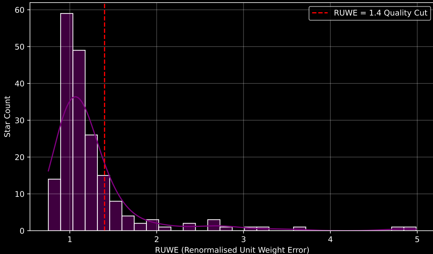
GAPOGEE DR17 Field [K2_C12_089-63_btx] RUWE Distribution (n= 192)
