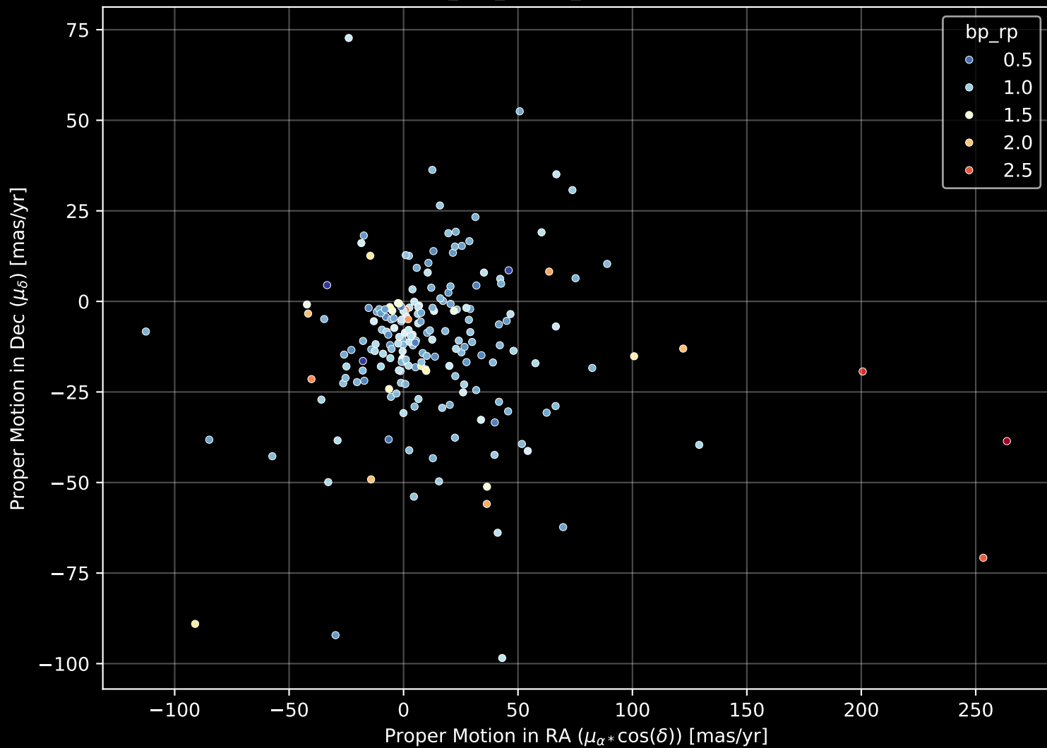
APOGEE DR17 Field: [K2_C12_089-63_btx] Proper Motion Diagram (n= 201)
